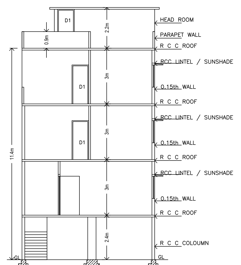
SECTION @ X-X
